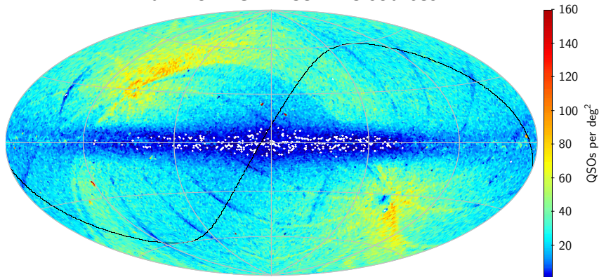
allWISE AGN: 1 354 775 sources
