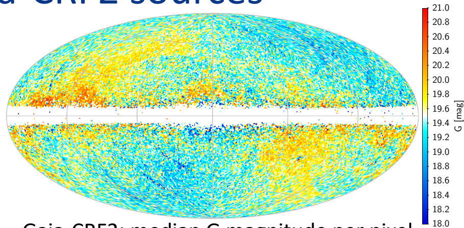
Gaia-CRF2: median G magnitude per pixel
