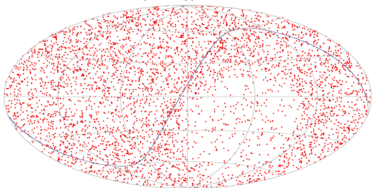
ICRF3 prototype: 4 262 sources
